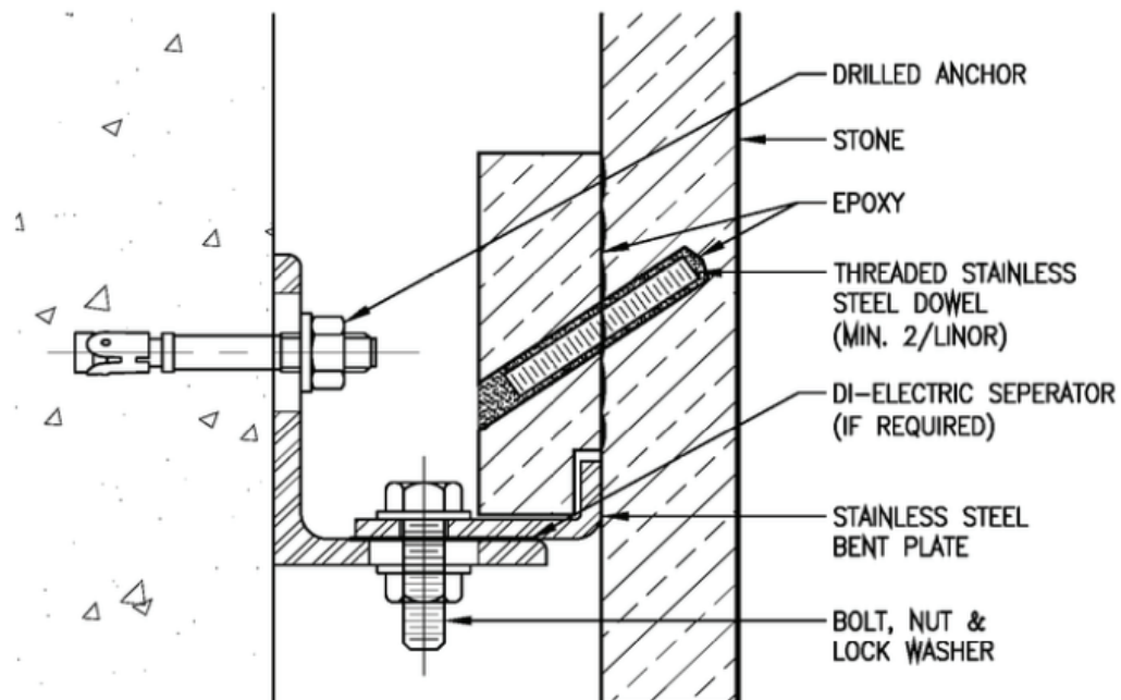
STONE LINER BLOCK CONNECTION
